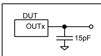
Figure 7. Test load
