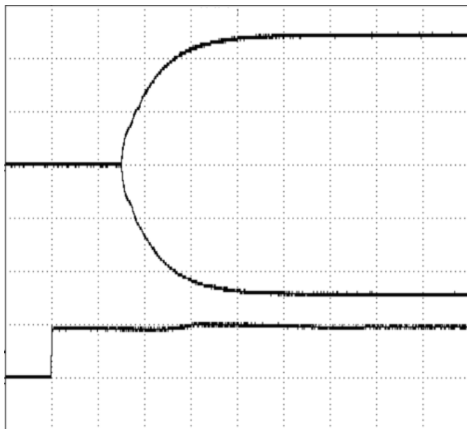
Figure 6: Turn-on transient at zero load current (5ms/div). V_{in}=48V . Top Trace: V_{out} : 5V/div; Bottom Trace: ON/OFF input: 50V/div
