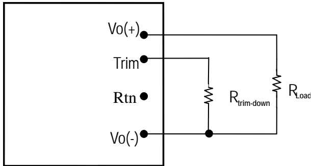
Figure 17: Circuit configuration for trim-down (decrease output voltage)
