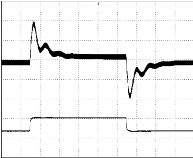
Figure 8: Output voltage response to step-change in load current I_{out1} (75%-50%-75% of I_o , max; di/dt = 0.1A/\mu s , 200uS/DIV). V_{in}=48V . Load cap: 10\mu F , tantalum capacitor and 1\mu F ceramic capacitor. Top trace: V_{out} (100mV/div), Bottom trace: I_{out} (1A/div). Scope measurement should be made using a BNC cable (length short than 20 inch). Position the load between 51 mm and 76 mm (2inch and 3 inch) from the module
