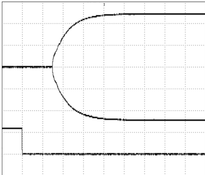
Figure 4: Turn-on transient at zero load current (5ms/div). V_{in}=48V . Top Trace: V_{out} : 5V/div; Bottom Trace: ON/OFF input: 5V/div
