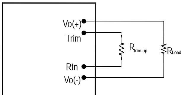
Figure 18: Circuit configuration for trim-up (increase output voltage)
