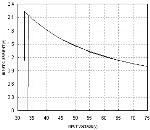
Figure 3: Typical input characteristics at room temperature (Io=full load)
