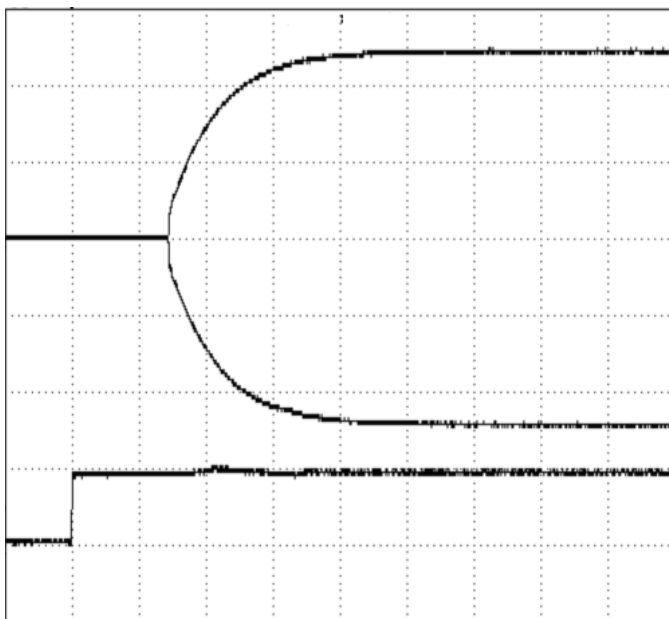
Figure 7: Turn-on transient at full rated load current (resistive load) (5 ms/div). V_{in}=48V . Top Trace: V_{out} ; 5V/div; Bottom Trace: ON/OFF input: 50V/div
