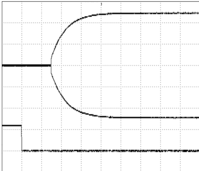
Figure 5: Turn-on transient at full rated load current (resistive load) (5 ms/div). V_{in}=48V . Top Trace: V_{out} ; 5V/div; Bottom Trace: ON/OFF input: 5V/div
