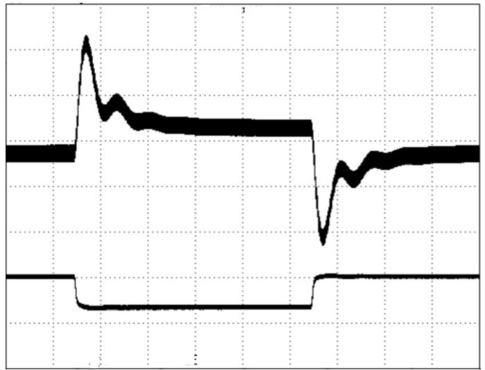
Figure 9: Output voltage response to step-change in load current I_{out2} (75%-50%-75% of I_o , max; di/dt = 0.1A/\mu s , 200uS/DIV). V_{in}=48V . Load cap: 10\mu F , tantalum capacitor and 1\mu F ceramic capacitor. Top trace: V_{out} (100mV/div), Bottom trace: I_{out} (1A/div). Scope measurement should be made using a BNC cable (length short than 20 inch). Position the load between 51 mm and 76 mm (2inch and 3 inch) from the module.
