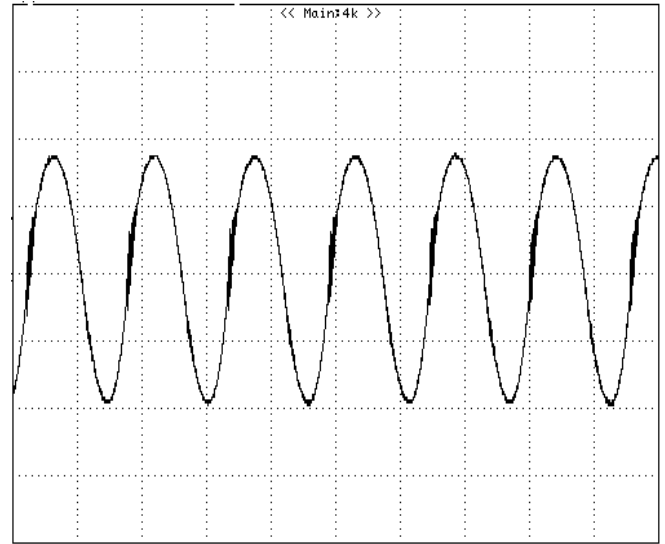
Figure 11: Input Terminal Ripple Current, i_C , at full rated output current and nominal input voltage with 12\ \mu\text{H} source impedance and 33\ \mu\text{F} electrolytic capacitor (200 mA/div).
