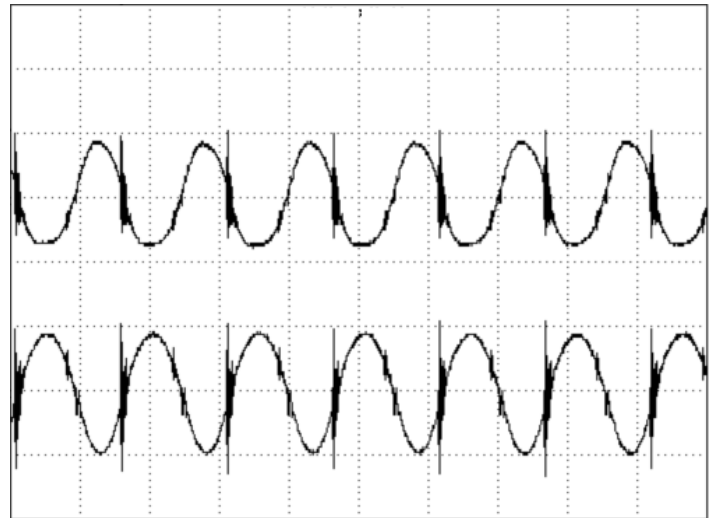
Figure 14: Output voltage ripple at nominal input voltage ( V_{in}=48V ) and rated load current ( I_{o1}=I_{o2}=2.7A ) (20 mV/div). Load capacitance: 1\mu F ceramic capacitor and 10\mu F tantalum capacitor. Bandwidth: 20 MHz. (See Figure 12). Scope measurement should be made using a BNC cable (length short than 20 inch). Position the load between 51 mm and 76 mm (2inch and 3 inch) from the module.
