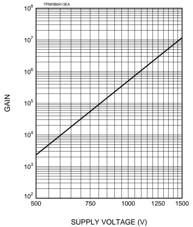
Figure 2: Typical Gain
