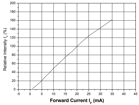
Relative Intensity I_v (%) vs Forward Current
