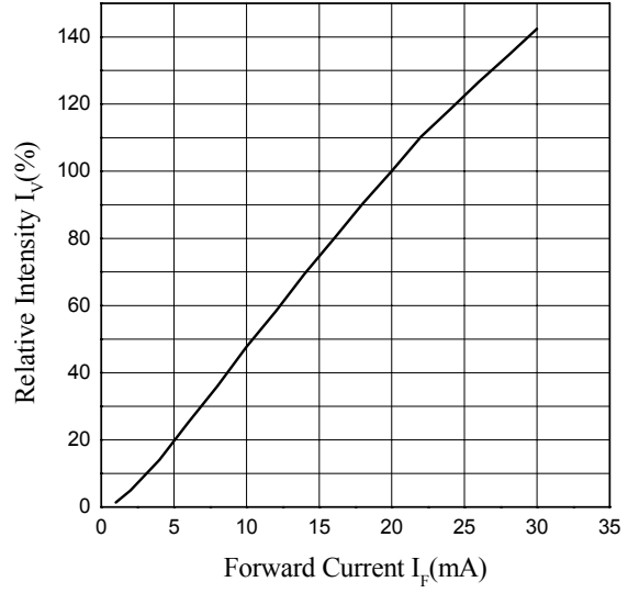
Relative Intensity I_v (%) vs Forward Current
