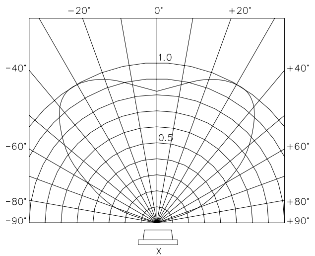
Radiation Diagram
