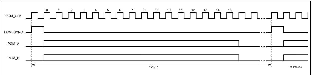
Figure 10. Linear mode
