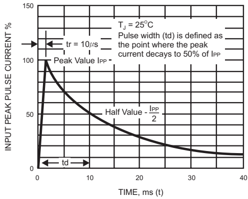
FIG.3- PULSE WAVEFORM
