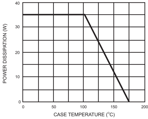
FIG.1- POWER DERATING CURVE
