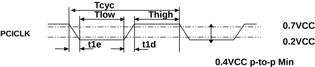
PCICLK Timing
