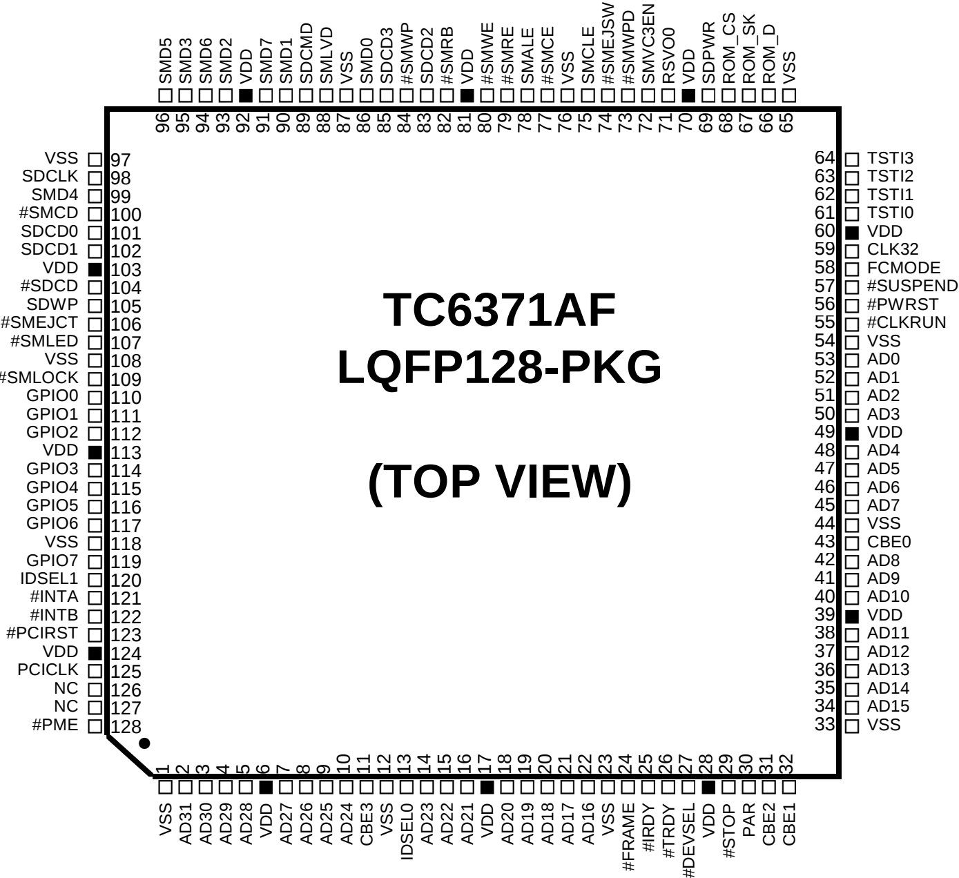
QFP128 Matrix Diagram
