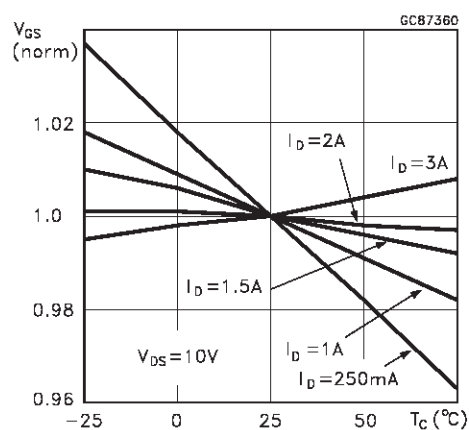
Gate-Source Voltage vs Case Temperature
