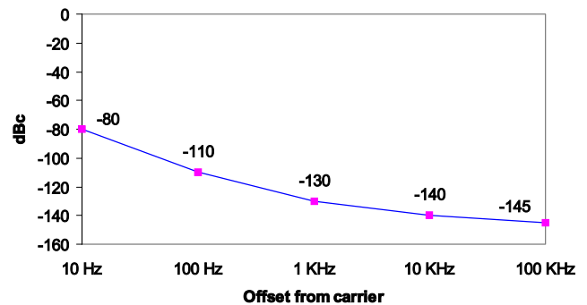
OVERTONE MODE (TYP. AT 50 MHz)
