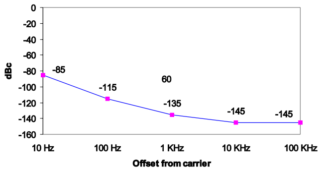
FUNDAMENTAL MODE (TYP. AT 10 MHz)
