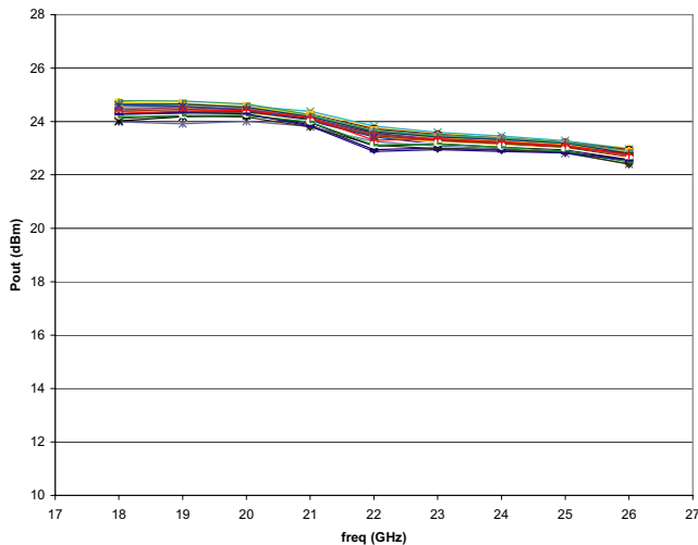
0289: Pout vs. freq, Pin = 0dBm
