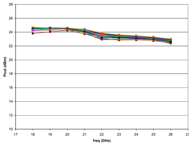
0289: Pout vs. freq Pin = 0dBm
