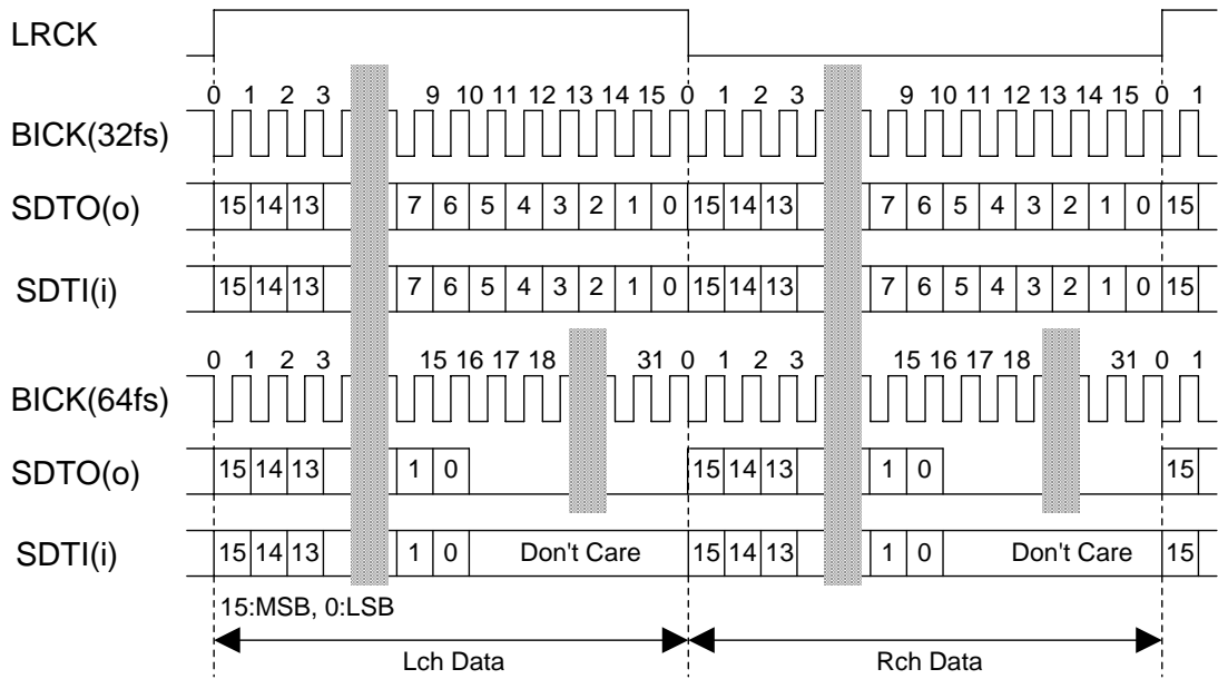
Figure 30. Mode 2 Timing
