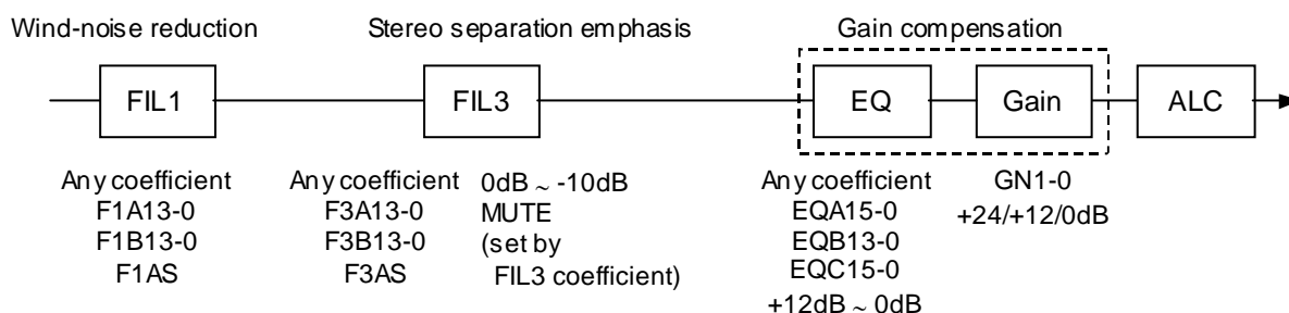
Figure 35. Digital EQ/HPF/LPF
