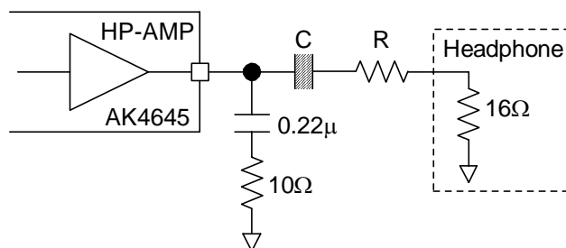
Figure 57. External Circuit Example of Headphone
