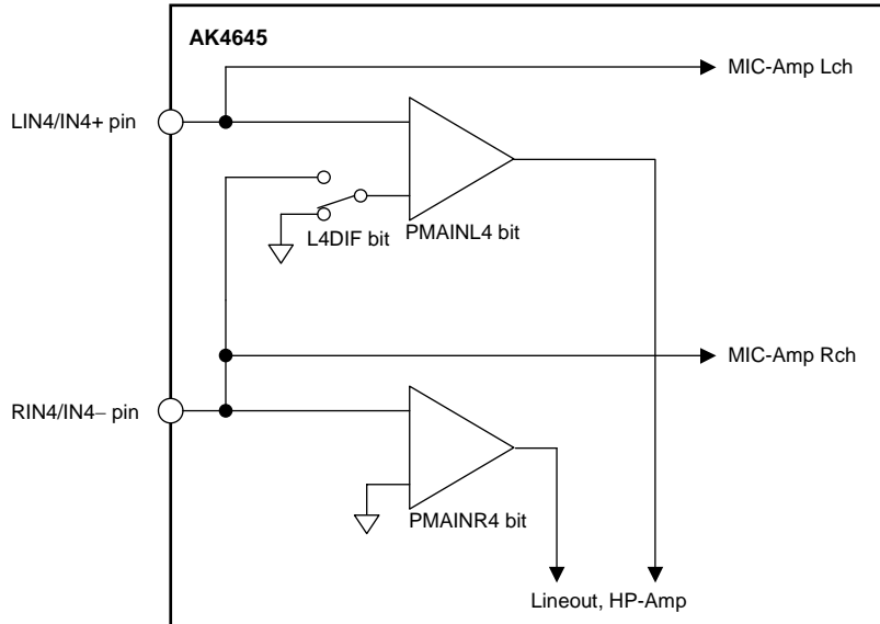
Figure 44. Full-differential Mono Analog Mixing Circuit
