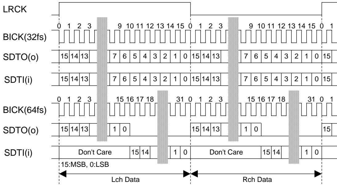
Figure 29. Mode 1 Timing
