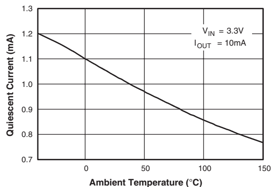
Ground Pin Current vs. Temperature
