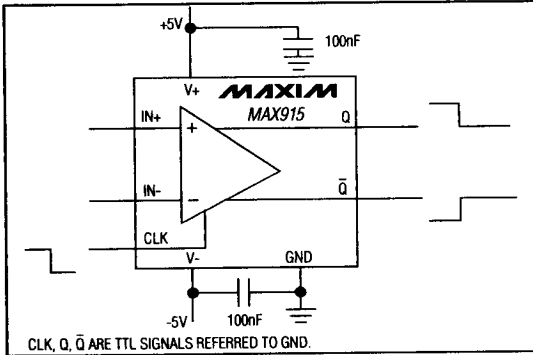
Figure 2. Dual-Supply Operation
