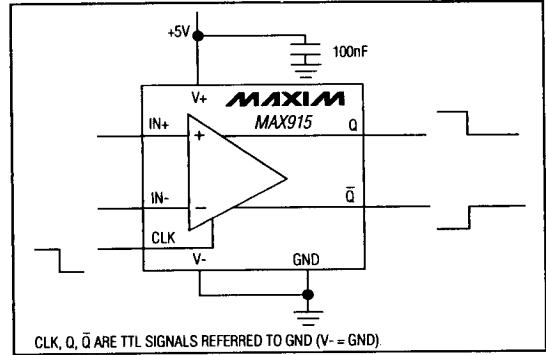
Figure 3. Single-Supply Operation
