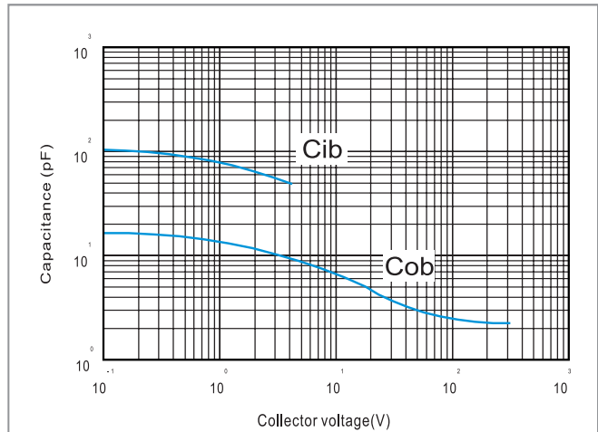
Fig.4 Capacitance
