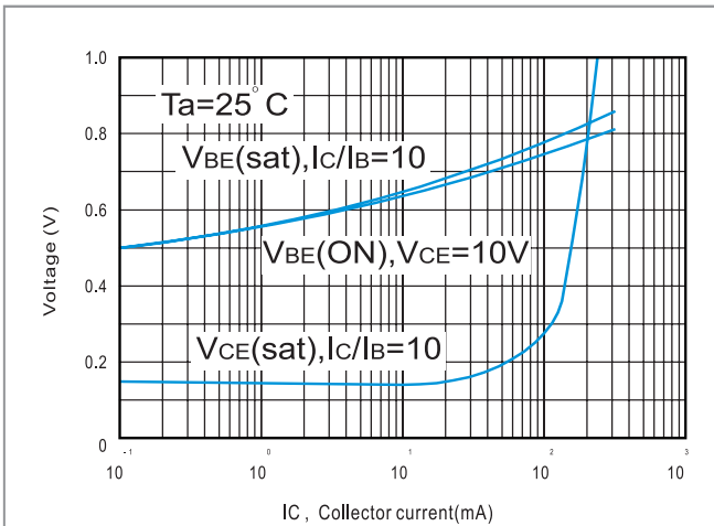
Fig.5 ON Voltage
