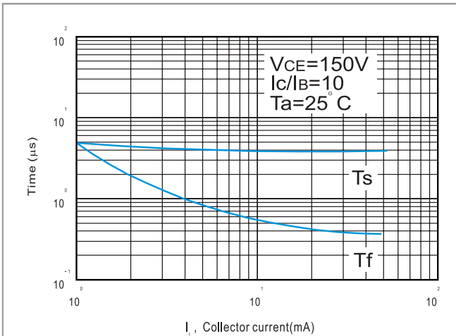
Fig.3 Turn-off switching time
