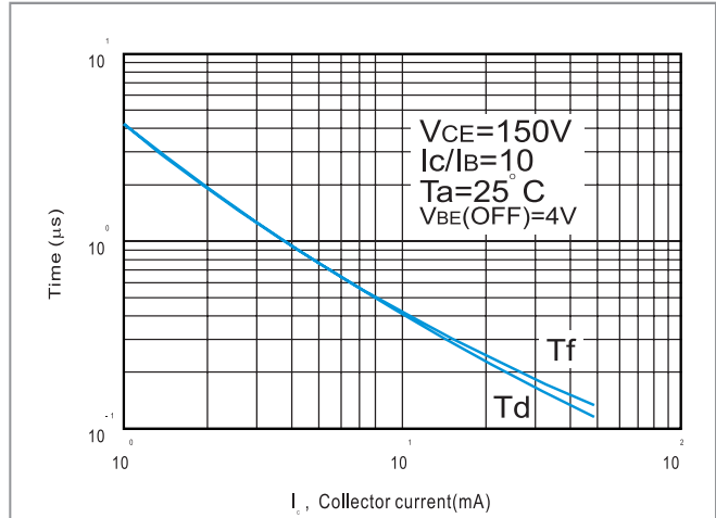
Fig.2 Turn-on switching time
