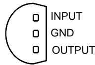
3-Pin Plastic TO-92 (Top View)
