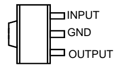
3-Pin Plastic SOT-89 Surface Mount (TOP View)
