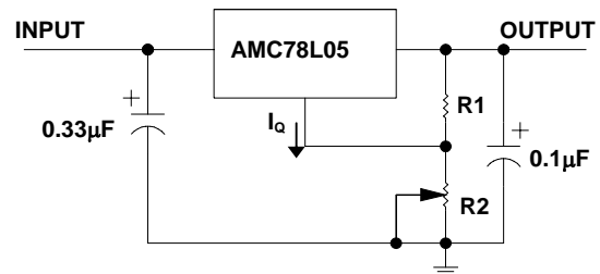
Fig. 2. Adjustable Output Regulator –
