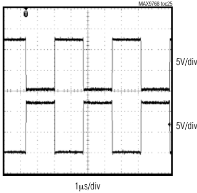
OUTPUT WAVEFORM (PWM MODE)
