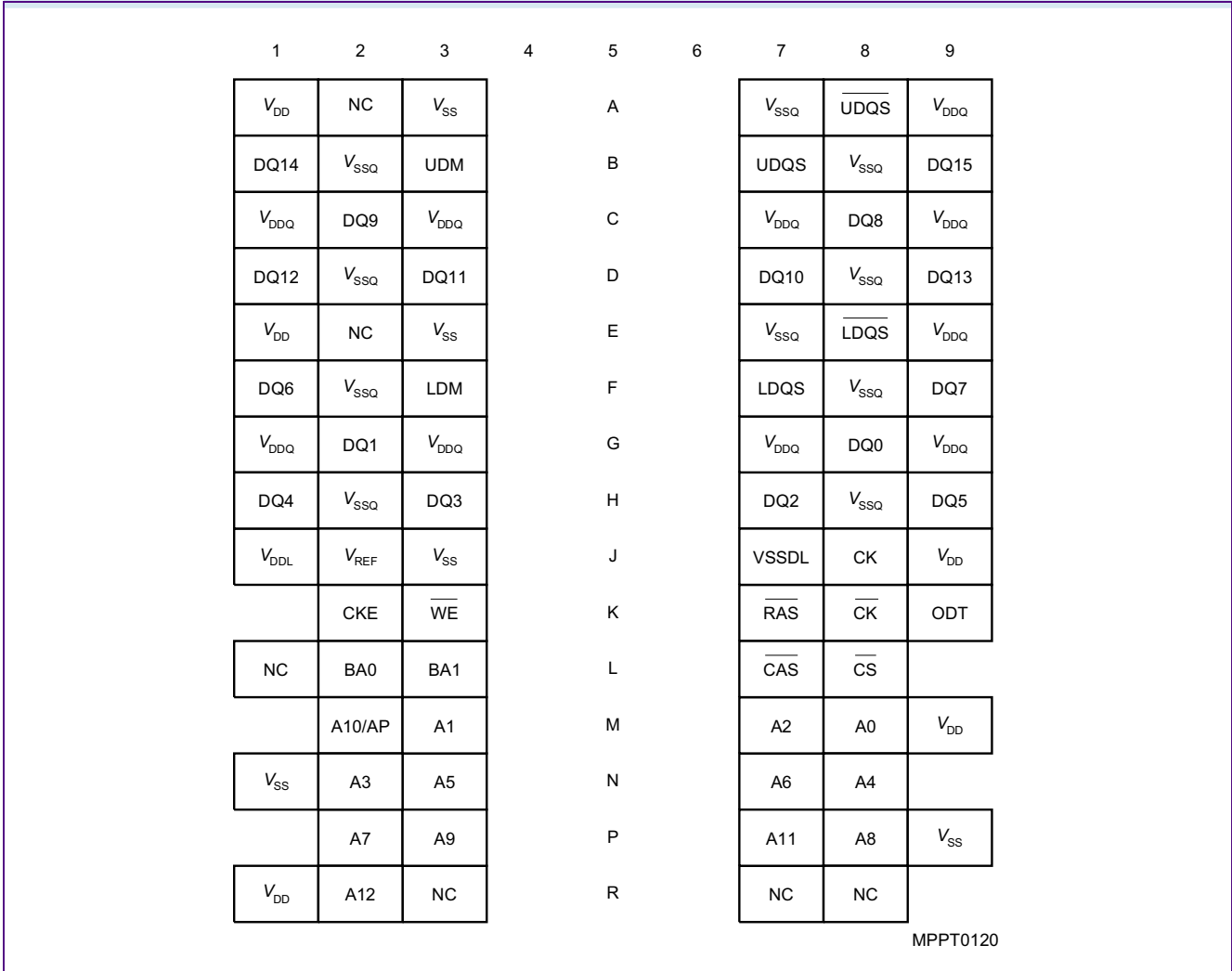
FIGURE 1 Chip Configuration for ×16 components, PG-TFBGA-84 (top view)
