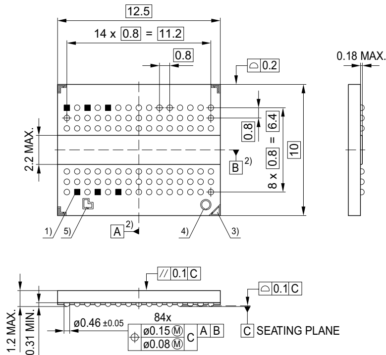
FIGURE 9 Package Outline PG-TFBGA-84
