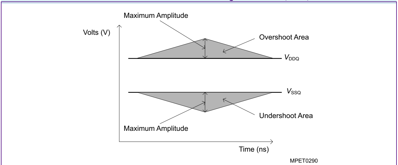
FIGURE 5 AC Overshoot / Undershoot Diagram for Clock, Data, Strobe and Mask Pins
