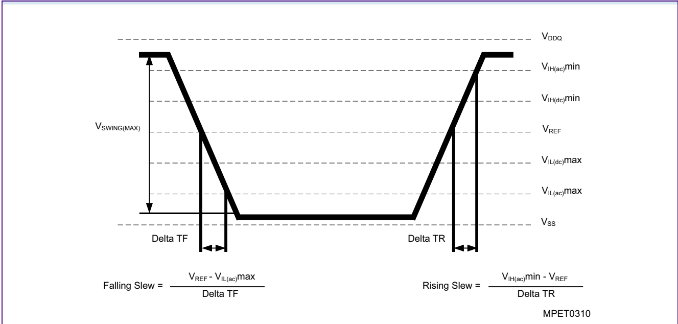
FIGURE 2 Single-ended AC Input Test Conditions Diagram
