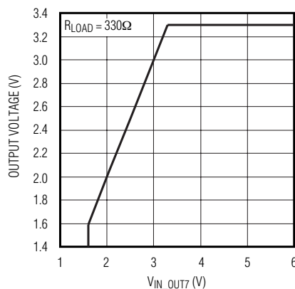
OUT7 REGULATOR LINE REGULATION
