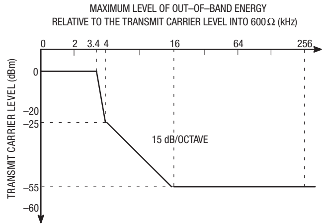
Figure 2. Out-of-Band Energy
