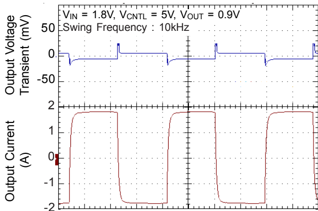
Time (25µs/Div)
