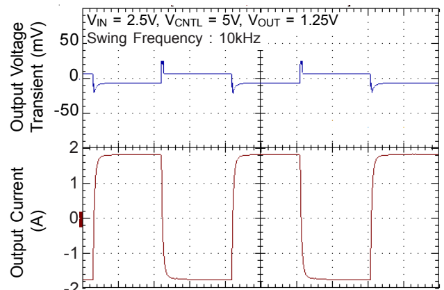
Time (25µs/Div)
