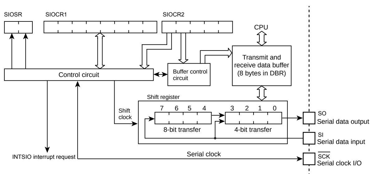
Figure 13-1 Serial Interface
