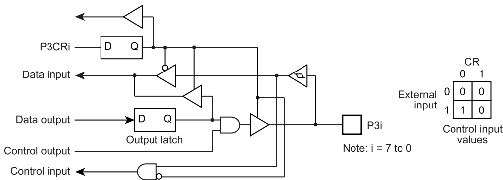
Figure 5-3 Port P3
