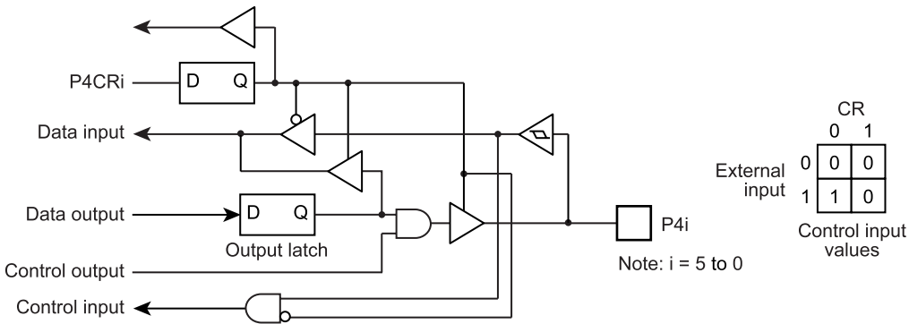
Figure 5-4 Port P4
