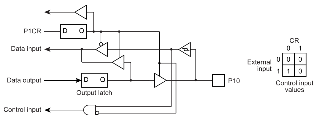
Figure 5-2 Port P1
