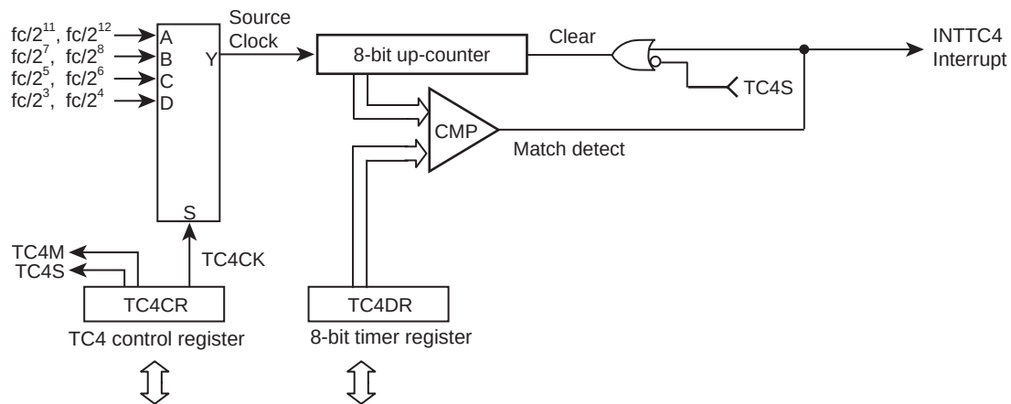
Figure 10-1 TimerCounter 4 (TC4)
