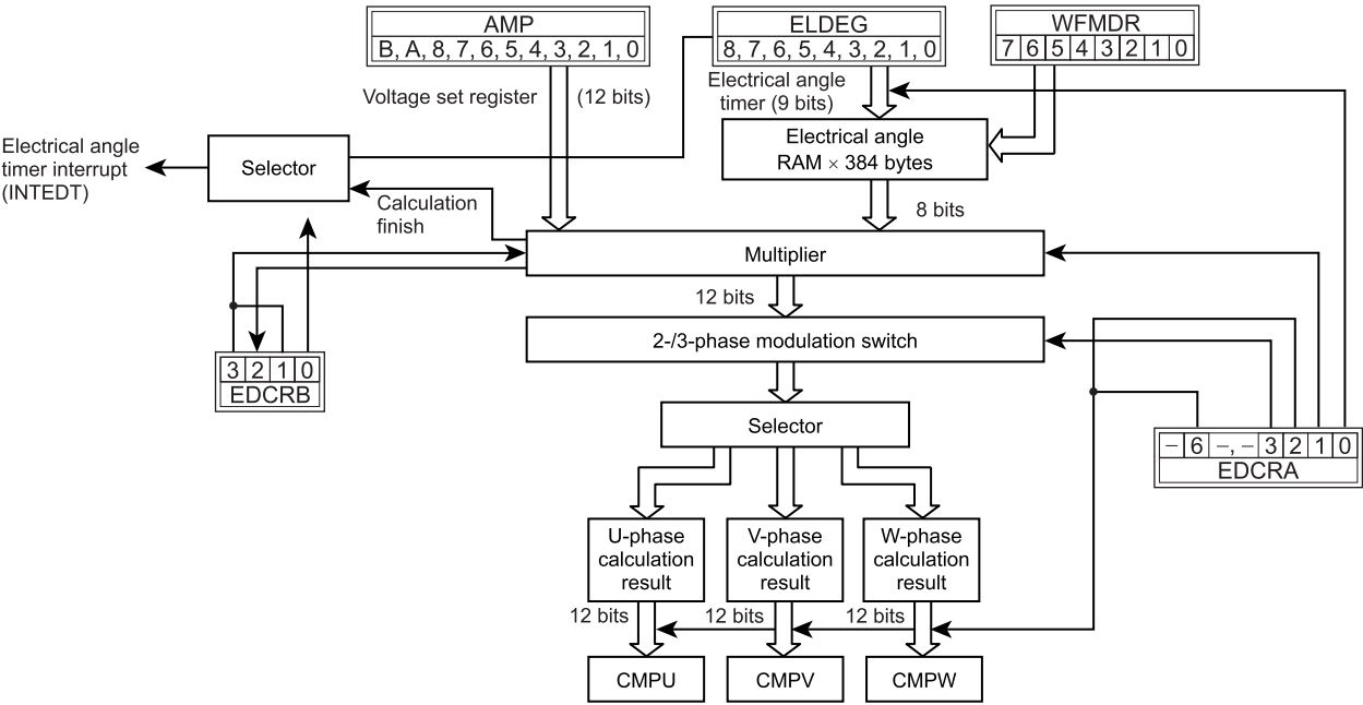
Figure 11-16 Waveform Arithmetic Circuit
