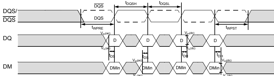
Figure 3 - Data Input (Write) Timing
