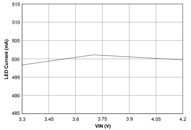
Spotlight Current, R_{ISET} = 750m\Omega , V_{OUT} = 2.93V
