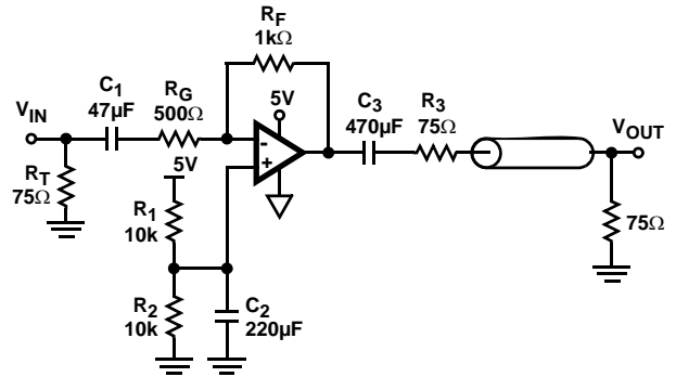
FIGURE 32. 5V SINGLE SUPPLY INVERTING VIDEO LINE DRIVER
