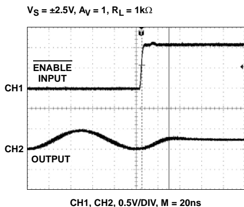
FIGURE 23. DISABLED RESPONSE
