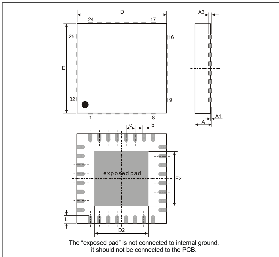
Fig 13: 32L QFN 5x5 Quad
