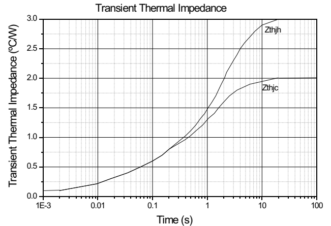
Fig. 6 - Transient Thermal Impedance Characteristics
