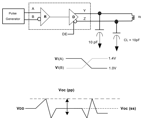
Figure 12. Test Circuit and Voltage Definitions for the Driver Common-Mode Output Voltage [[6],[7],[8],[9]]
