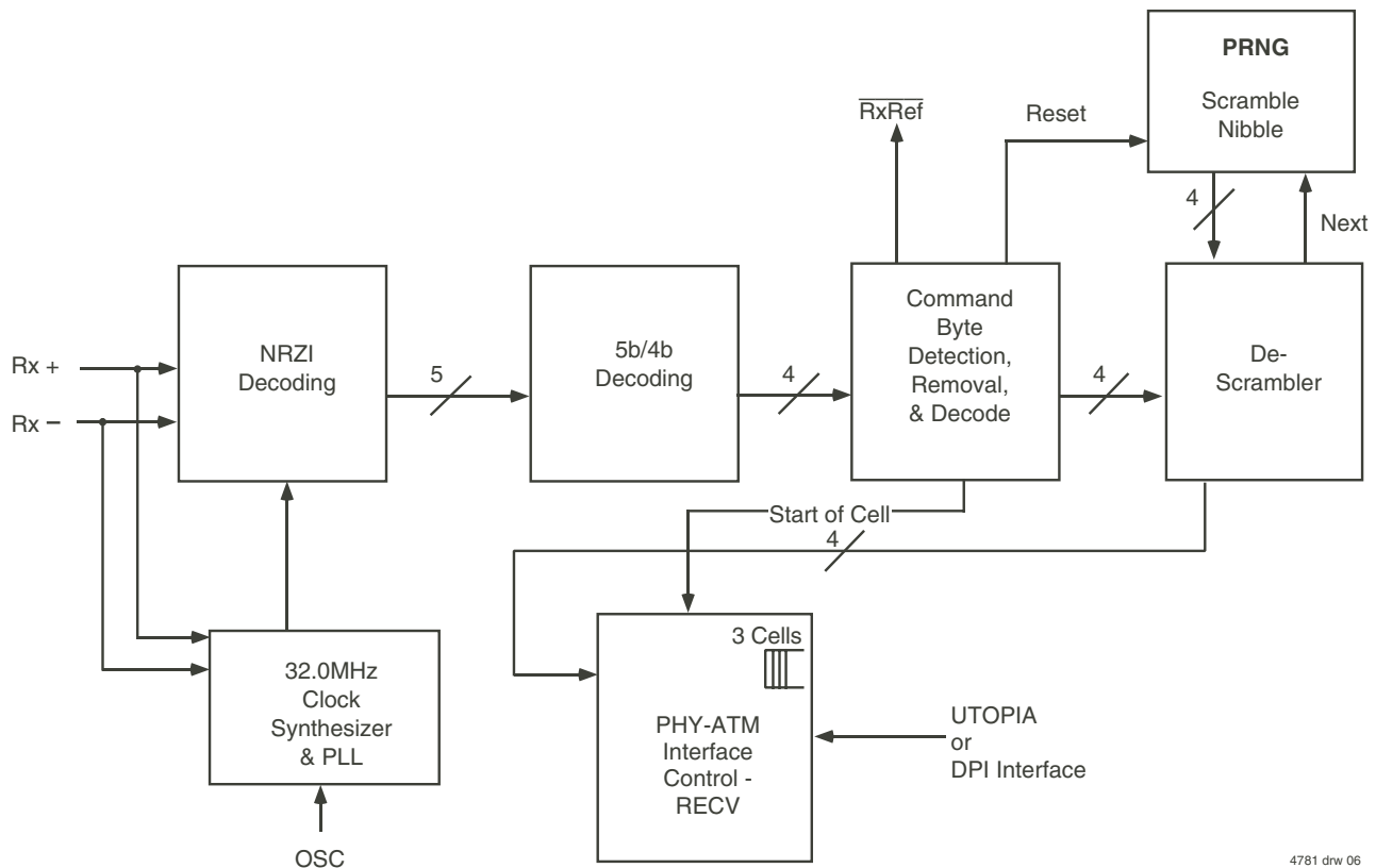
Figure 5. TC Receive Block Diagram
