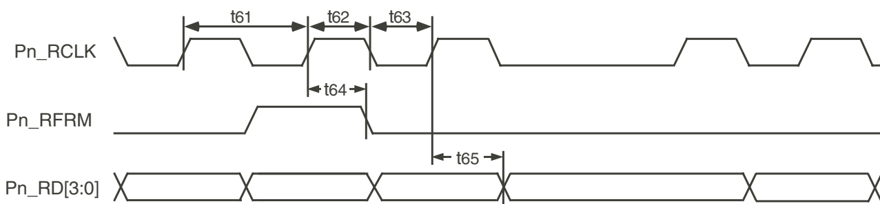
Figure 41. DPI Receive
