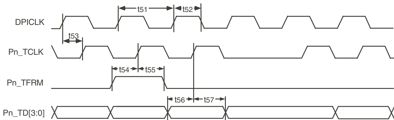
Figure 40. DPI Transmit
