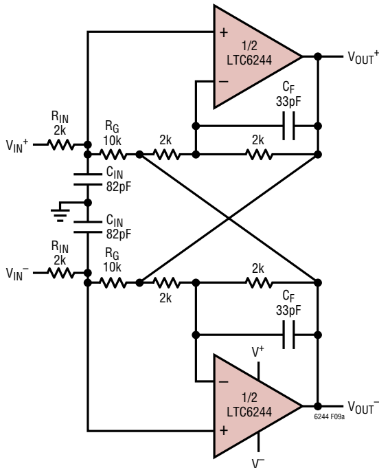
Figure 9a. Low Noise Fully Differential Buffer/Amplifier (f -3dB = 970kHz, Gain = 5, R IN = 4k)
