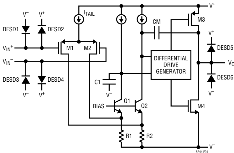
Figure 1. Simplified Schematic
