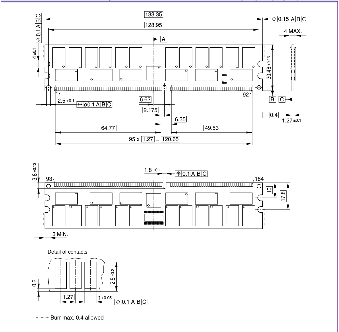
Package Outlines – Raw Card D HYS72D128320[G/H]BR-[6/7]-C (2 Ranks ×4)
