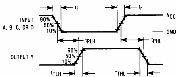
Figure 1. Switching Waveforms
