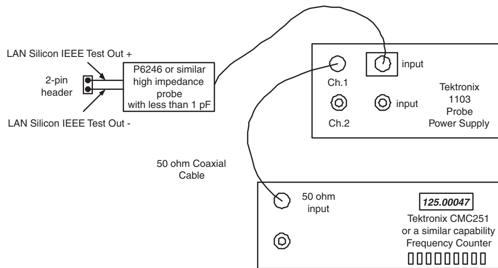
Figure 11. Indirect Probing Setup
