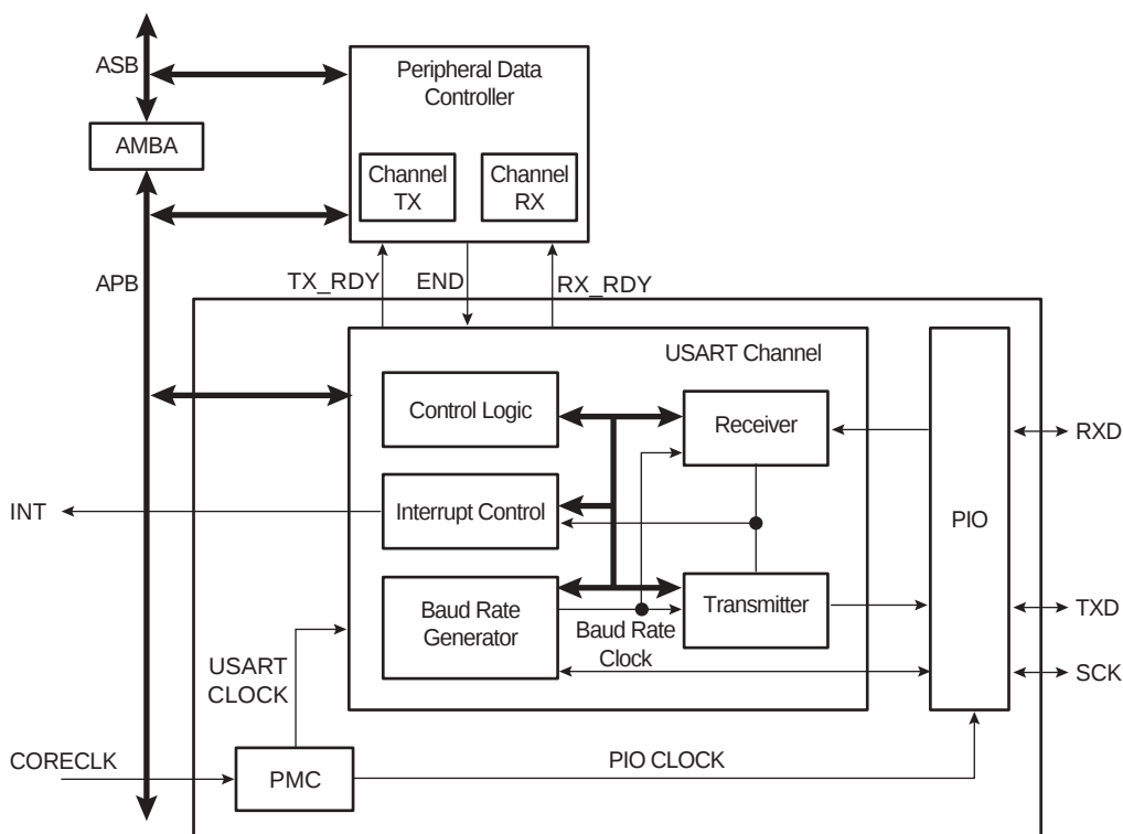
Figure 49. USART Block Diagram
