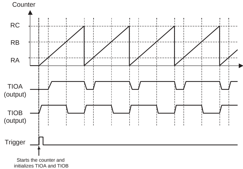
Figure 97. Dual Pulse Width Modulation
