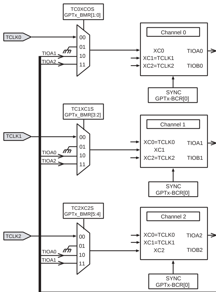
Figure 104. Timer Controller Block Programming Diagram
