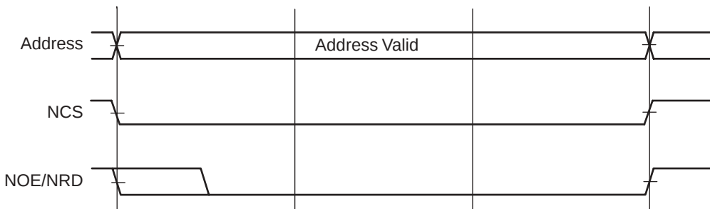
Figure 20. Read Cycle with Two Wait States
