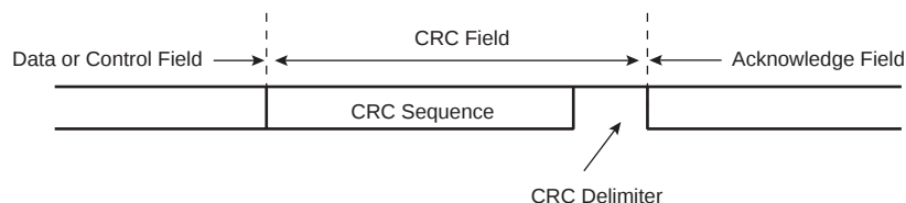
Figure 79. CRC Field
