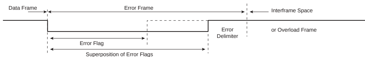
Figure 82. Error Frame
