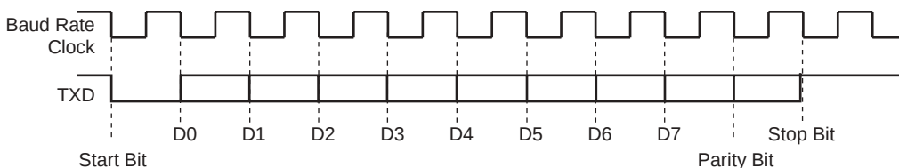
Figure 55. Synchronous and Asynchronous Modes, Character Transmission
