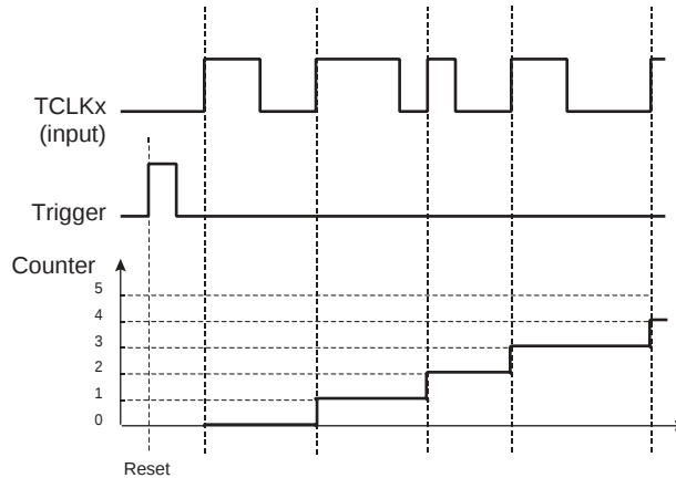
Figure 101. Event Counter
