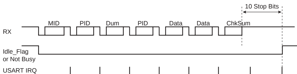
Figure 54. Idle Flag
