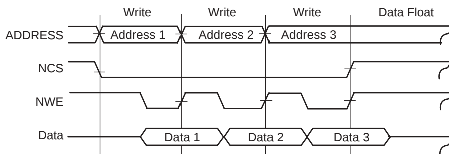
Figure 33. Sequential Write Access on the Same Chip Select with No Wait State
