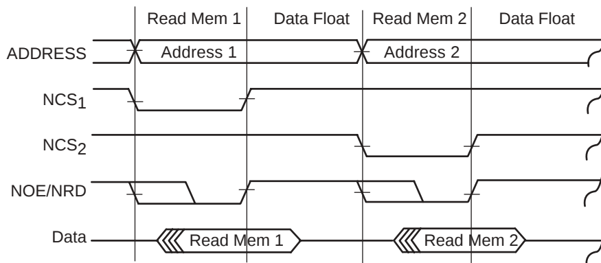
Figure 29. Sequential Read Access on Different Chip Select with NTDF = 0 or 1
