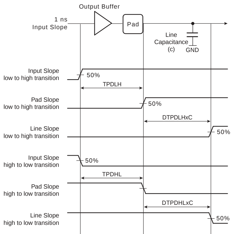
Figure 3. Propagation Delay
