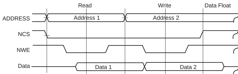
Figure 32. Sequential Write Access on the Same Chip Select with One Wait State
