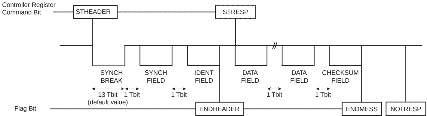
Figure 56. Message Characteristics
