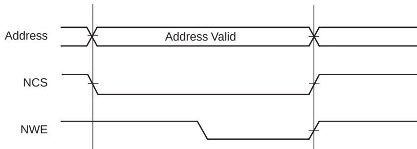
Figure 18. Write Access
