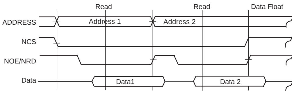
Figure 30. Sequential Standard Read Access on the Same Chip Select with One Wait State
