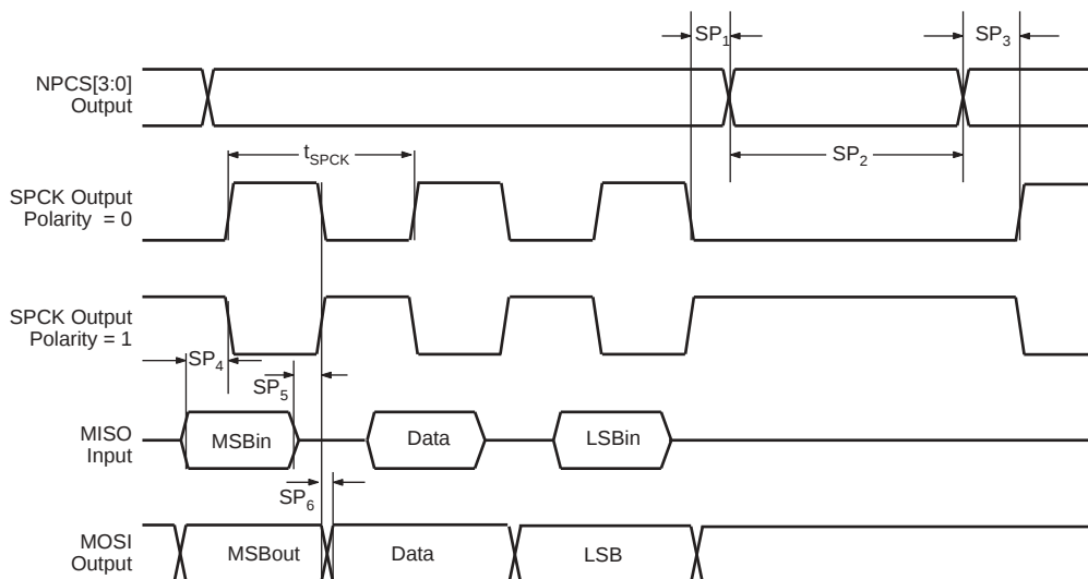
Figure 69. SPI Timings
