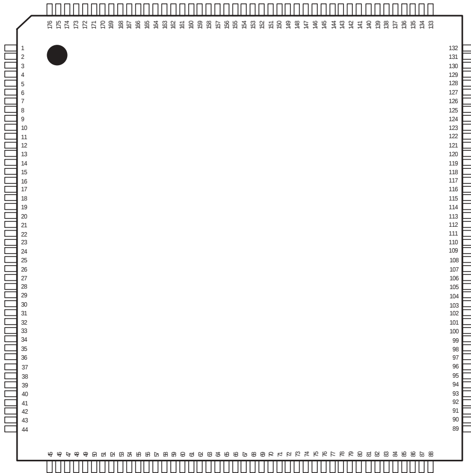
Figure 1. Pin Configuration
