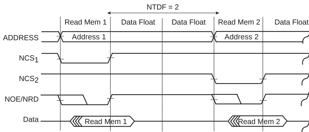
Figure 28. Sequential Read Access on Different Chip Select with NTDF = 2
