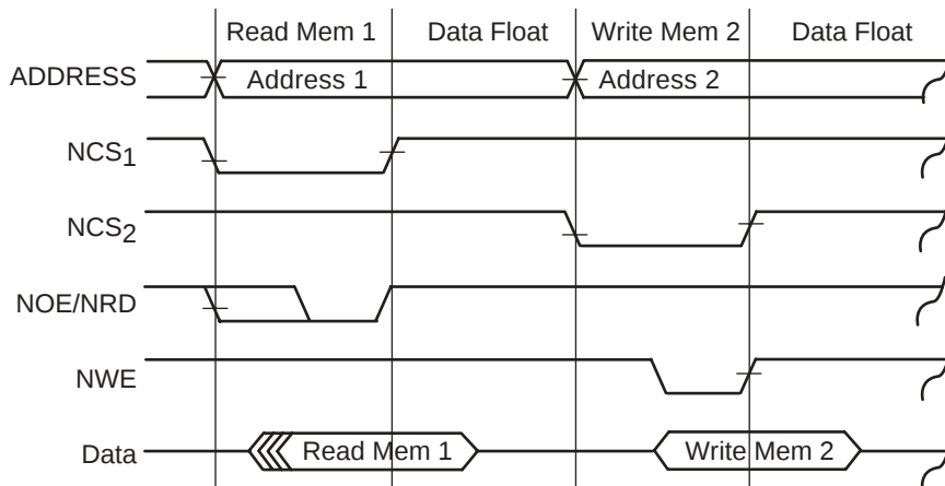
Figure 23. Read and Write Access on Different Chip Select with NTDF = 0 or 1
