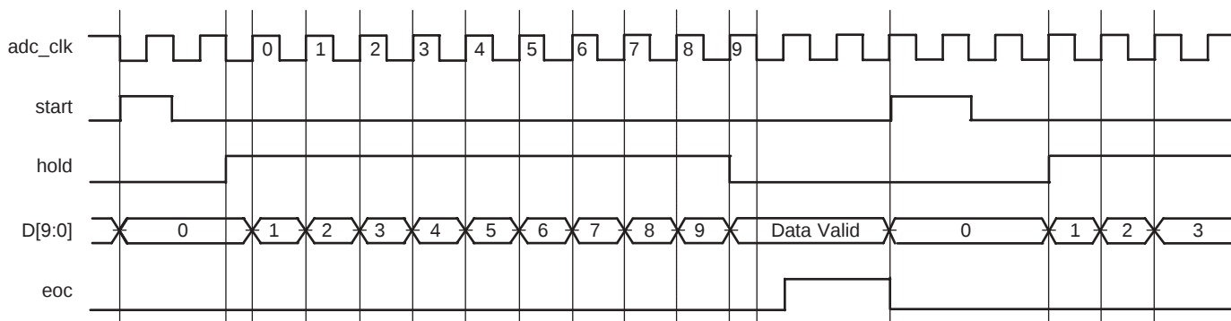
Figure 47. Signal Description
