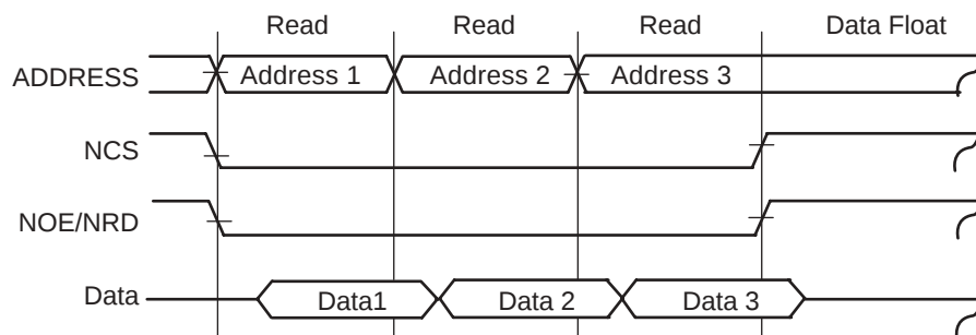
Figure 27. Sequential Early Read Access on the Same Chip Select with No Wait State
