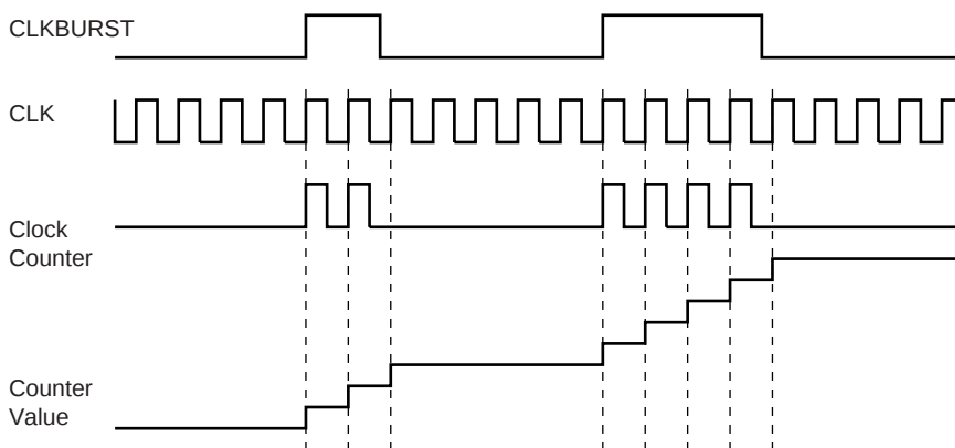
Figure 90. Burst Clock
