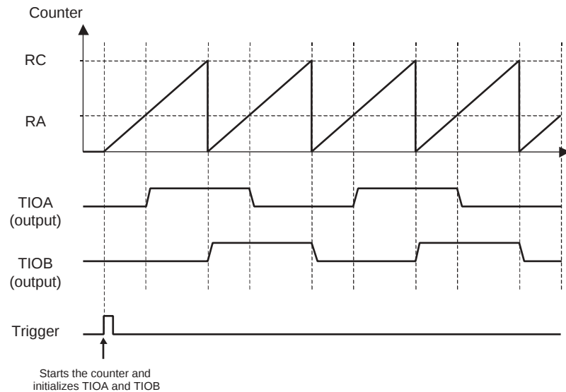
Figure 98. Two Square Signals
