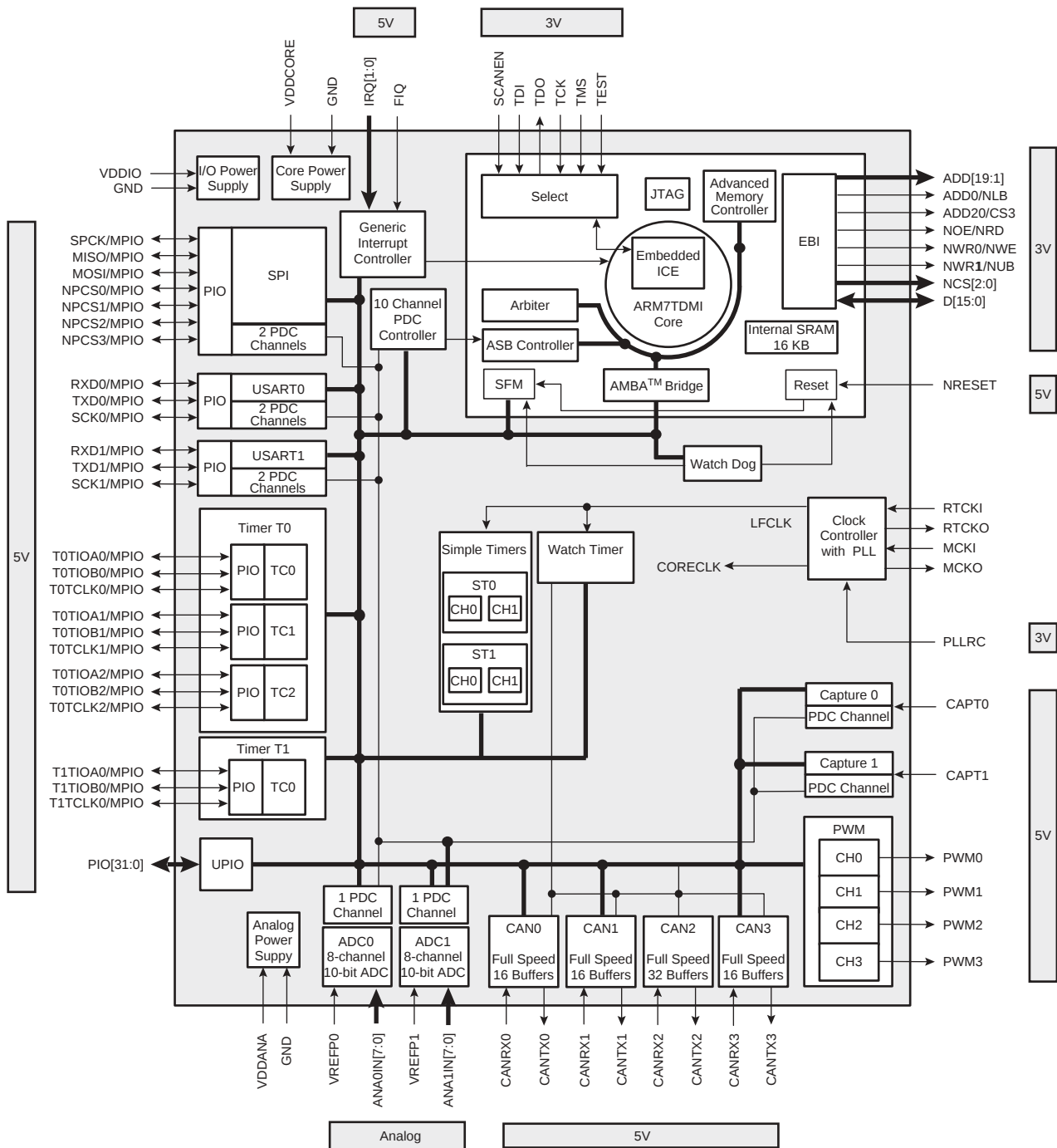
Figure 2. Block Diagram
