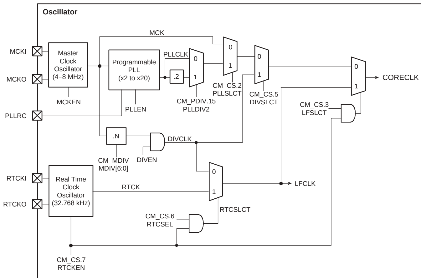
Figure 40. Clock Management
