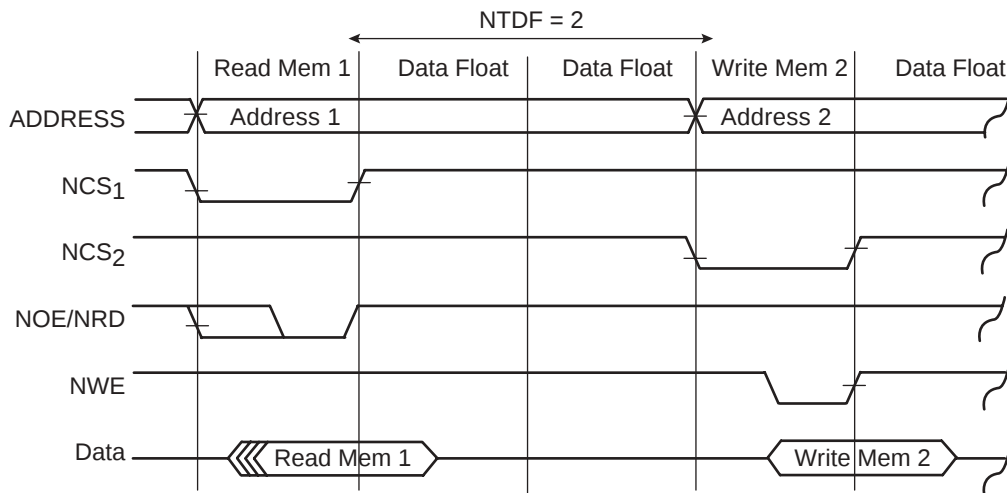
Figure 24. Read and Write Access on Different Chip Select with NTDF = 2
