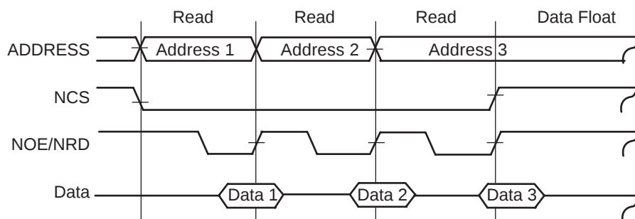
Figure 31. Sequential Standard Read Access on the Same Chip with No Wait State
