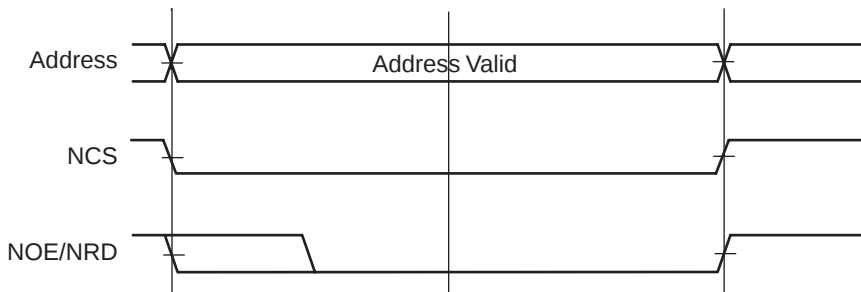
Figure 19. Read Cycle with One Wait State
