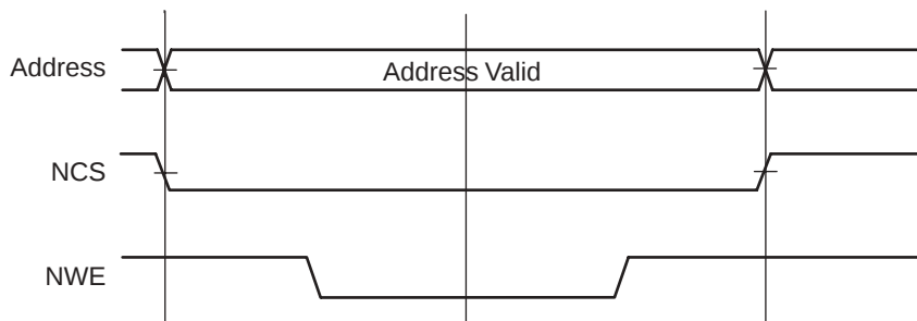
Figure 21. Write Cycle with One Wait State
