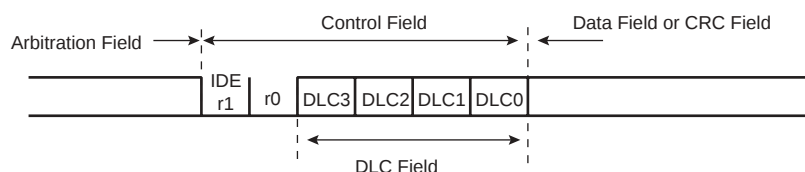
Figure 78. Control Field
