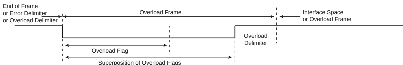
Figure 83. Overload Frame
