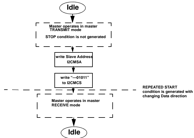
Figure 13-11. Master Burst RECEIVE after Burst SEND
