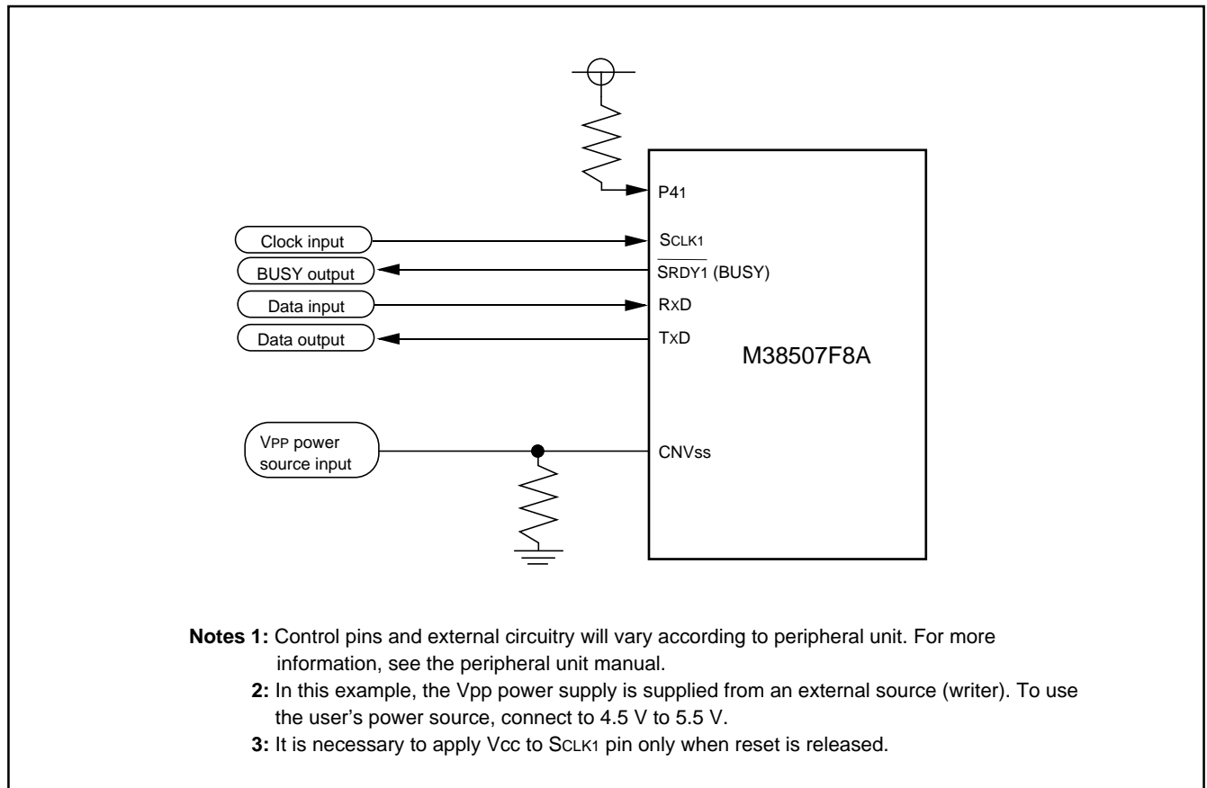
Fig. 66 Example circuit application for standard serial I/O mode
