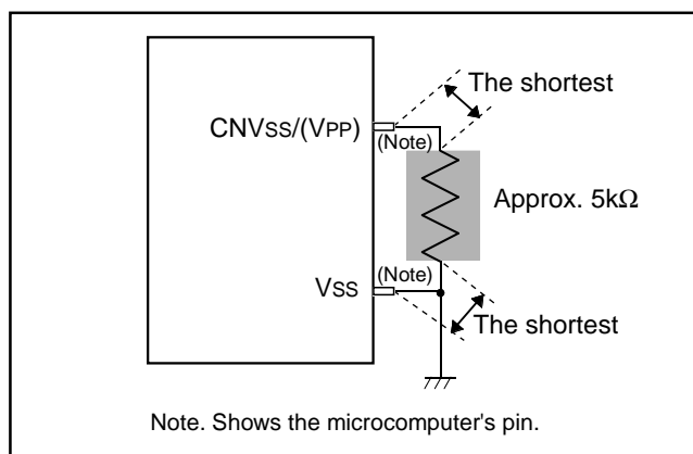
Fig. 7 Wiring for the CNVSS/VPP pin
