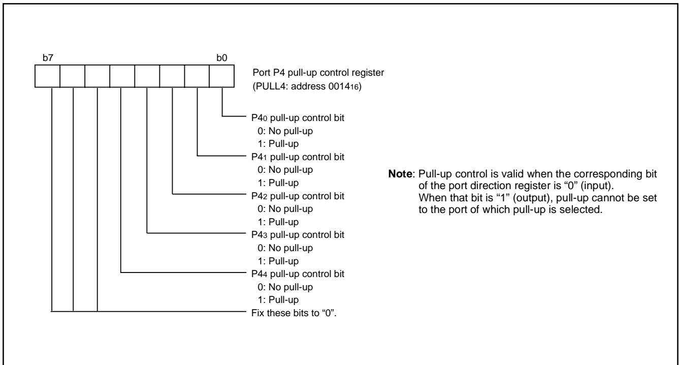
Fig. 14 Structure of port registers (2)
