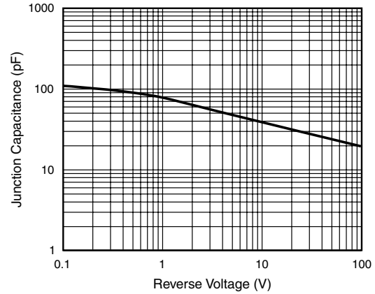
Figure 5. Typical Capacitance
