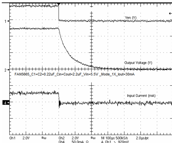
Figure 26. Turn-off at I_{OUT} = 30mA in 1x Mode
