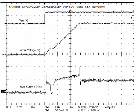
Figure 27. Start-up at I_{OUT} = 30mA in 1.5x Mode
