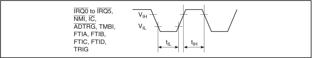
Figure 29.5 Input Timing
