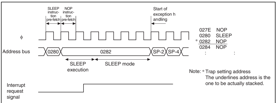
Figure 27.18 SLEEP Instruction (3)
