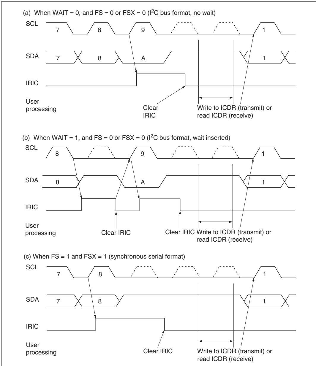
Figure 25.12 IRIC Setting Timing and SCL Control
