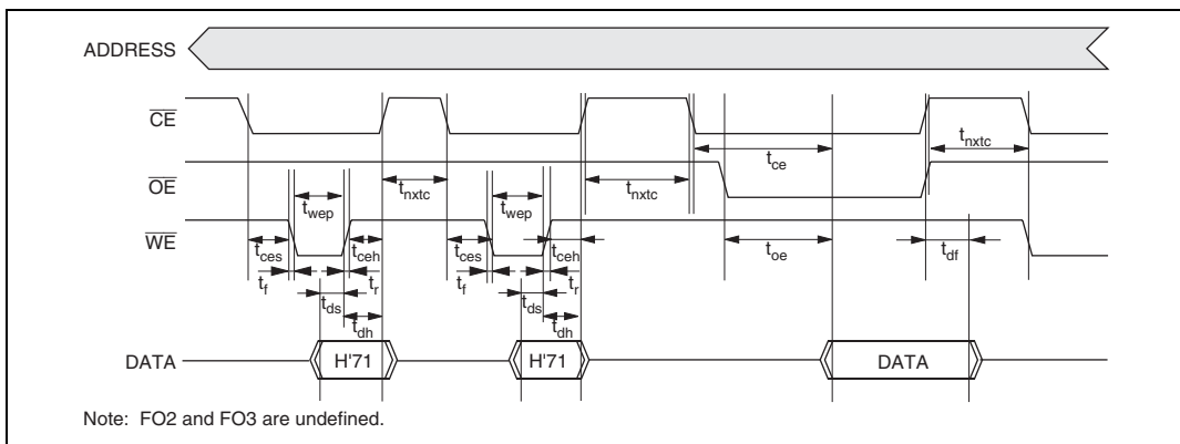
Figure 7.22 Status Read Mode Timing Waveforms
