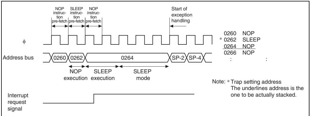
Figure 27.17 SLEEP Instruction (2)
