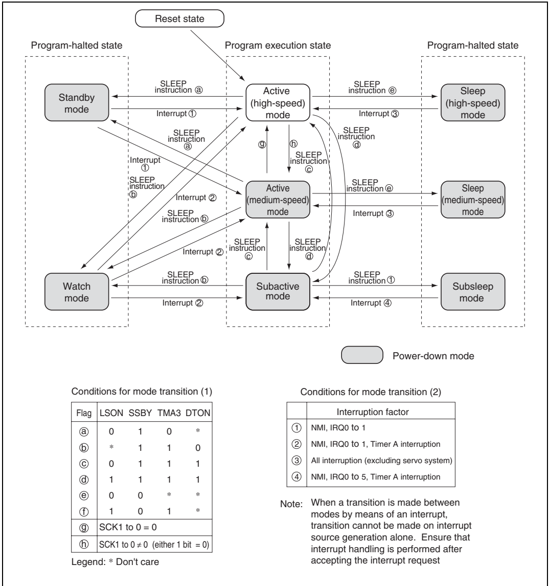
Figure 4.1 Mode Transitions
