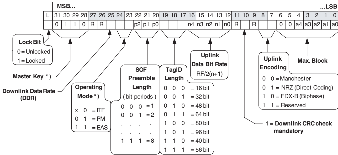
Figure 2-7. Configuration Register
