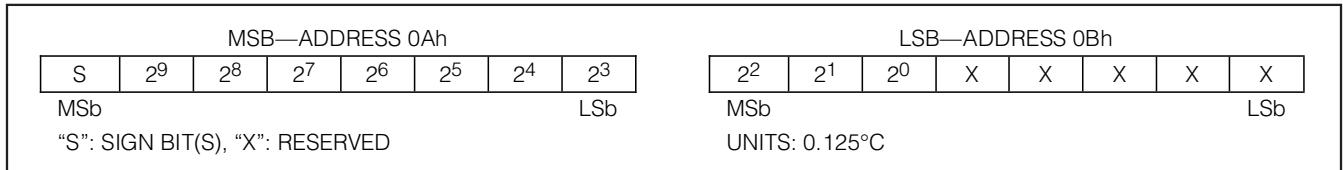
Figure 5. Temperature Register Format
