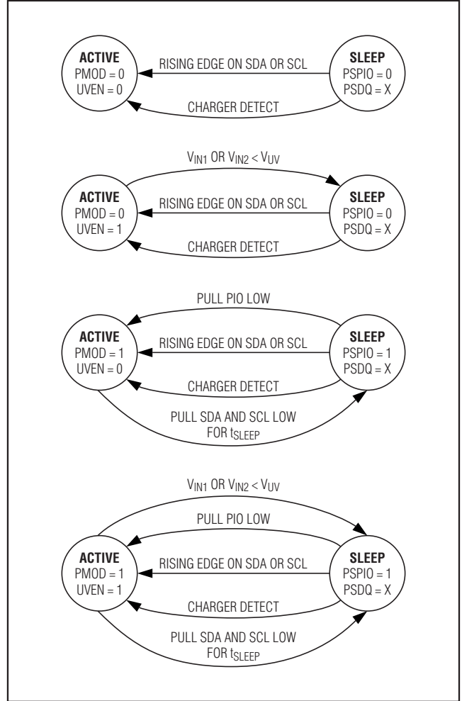
Figure 2. Sleep-Mode State Diagram for DS2777/DS2778
