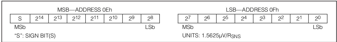
Figure 6. Current Register Format
