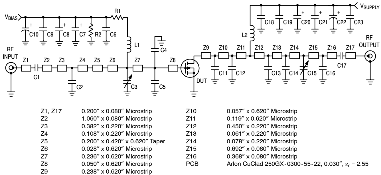
Figure 1. MRFE6S9125NR1(NBR1) Test Circuit Schematic
