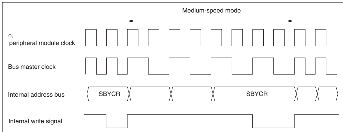
Figure 21.2 Medium-Speed Mode Transition and Clearance Timing
