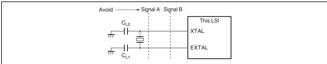
Figure 20.9 Note on Board Design of Oscillator Circuit
