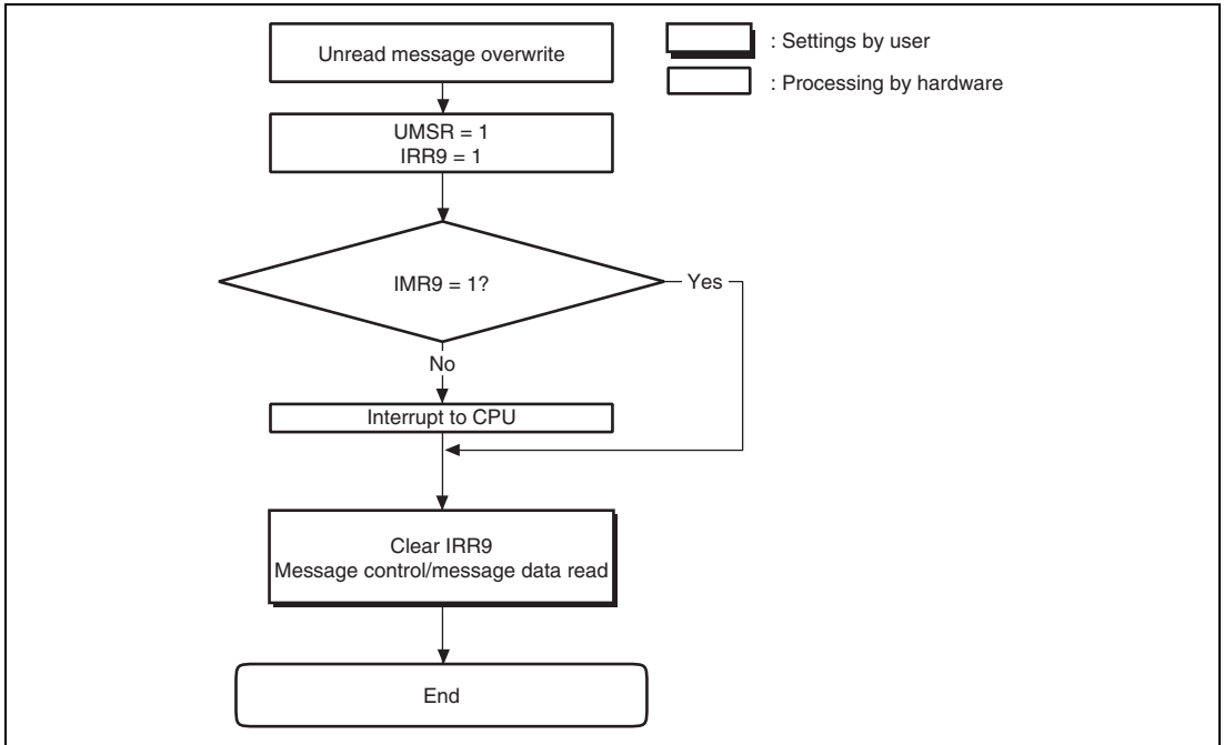
Figure 14.12 Unread Message Overwrite Flowchart
