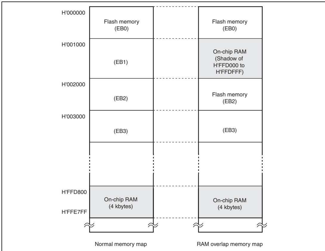
Figure 19.8 Example of RAM Overlap Operation
