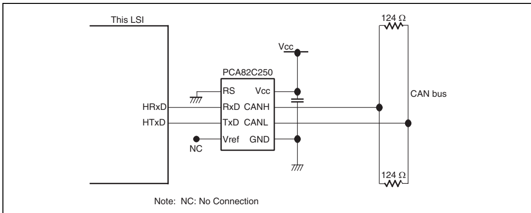
Figure 14.16 High-Speed Interface Using PCA82C250
