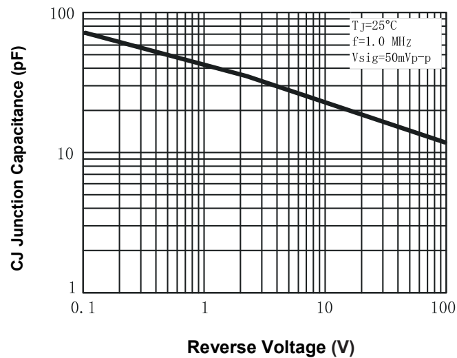
Fig.5- Junction Capacitance
