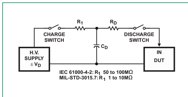
Figure 1: Electrostatic Discharge Test
