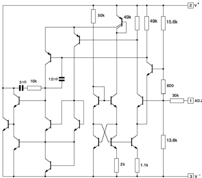
Figure 2 - circuitry IL135Z.
