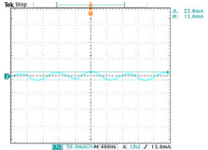
Figure 27. Input reflected ripple current \dot{I}_s waveform With 10uH input inductor. At V_{in}=48v , I_{out}=25A , 50ma/Div ( current probe with 50mv/div)
