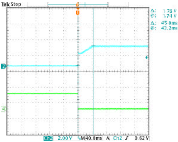
Figure 12. Turn on timing vs. Input On/Off Pin. Waveform 2 is output voltage, waveform 4 is negative On/Off logic signal. At 48v input voltage, 20A output current with 100uf output capacitance load.
