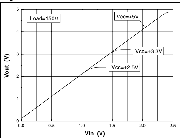
Figure 4. Distortion
