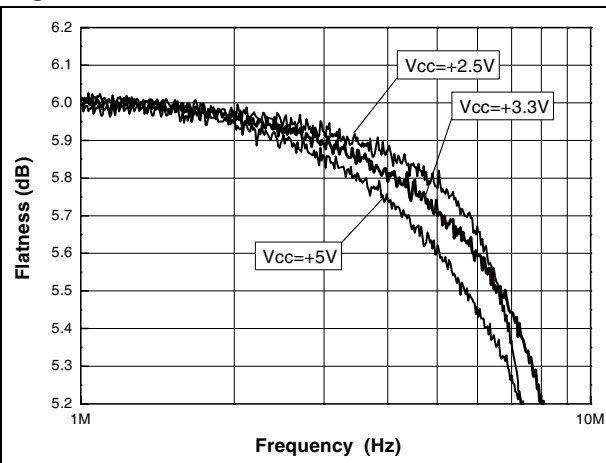
Figure 2. Gain flatness
