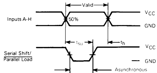
Figure 4. Parallel-Load Mode
