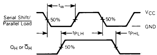
Figure 2. Parallel-Load Mode
