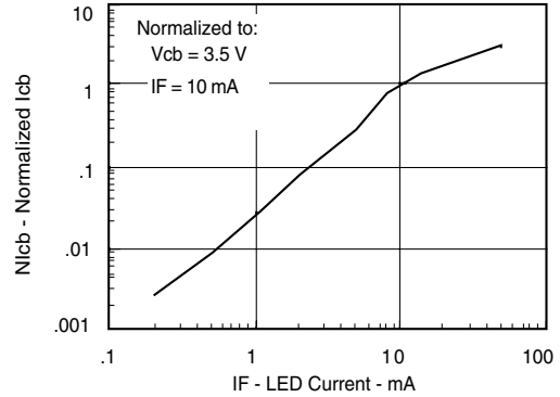
Fig. 4 - Normalized Collector Base Photocurrent vs. LED Current
