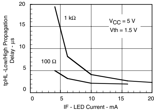
Fig. 7 - High to low Propagation Delay vs. Collector Load Resistance and LED Current
